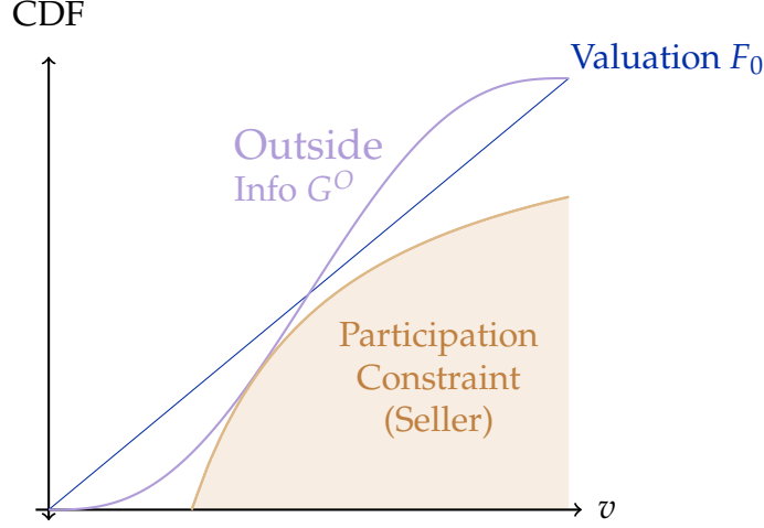
Figure 7: Participation constraint: profits on the platform must weakly exceed profits under outside information.
