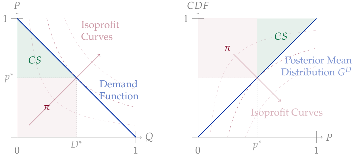
Figure 1: Sellers Optimal Price Setting Strategy
