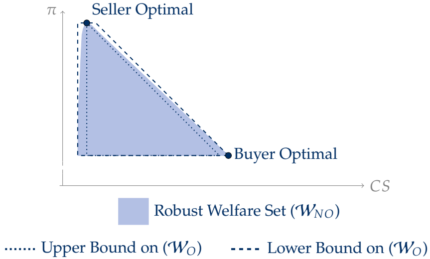
Figure 6: Robust Welfare Set and Bounds on Welfare Outcomes
